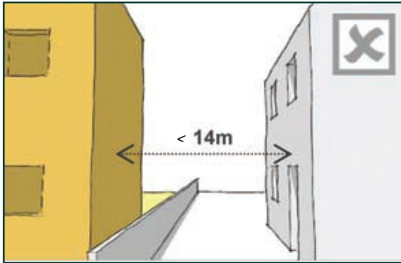
Figure 17: Distance of 14.00 metres between a protected window and a blank two-storey wall
