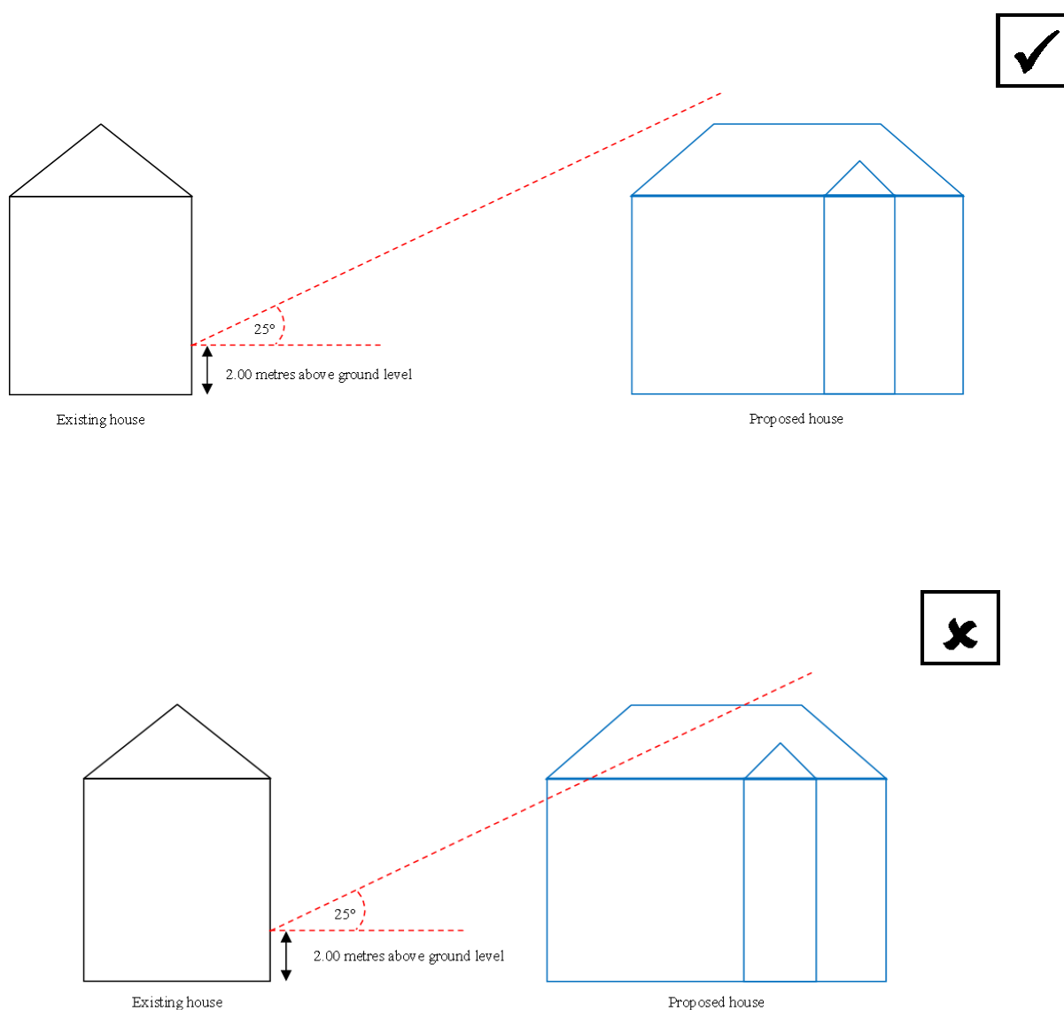
Figure 13: 25° test for natural light (elevations)
